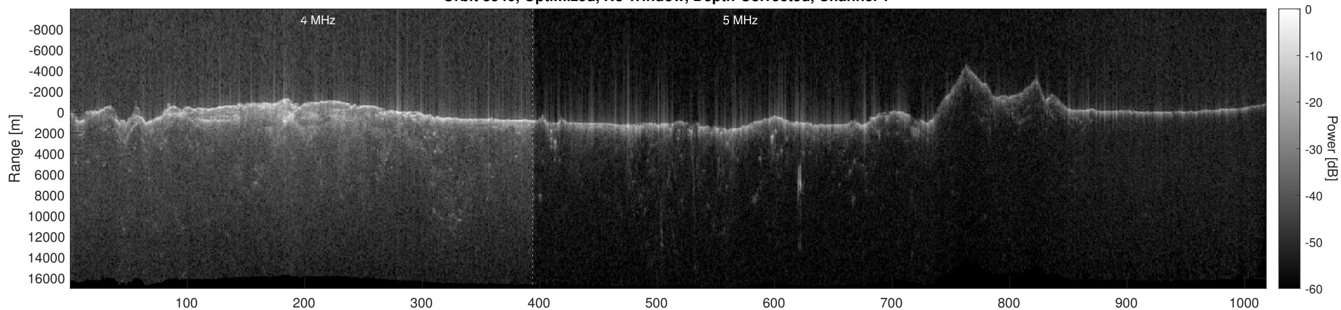
Orbit 8540, Optimized, No Window, Depth-Corrected, Channel 2
