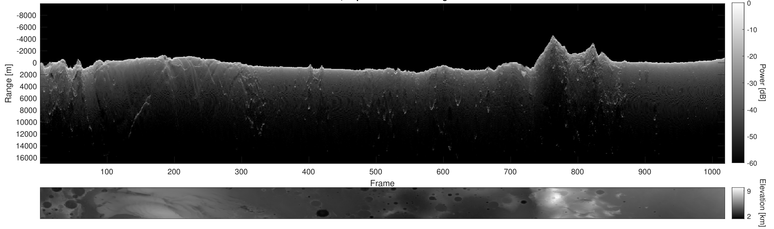
Orbit 8540, Depth-Corrected Cluttergram
