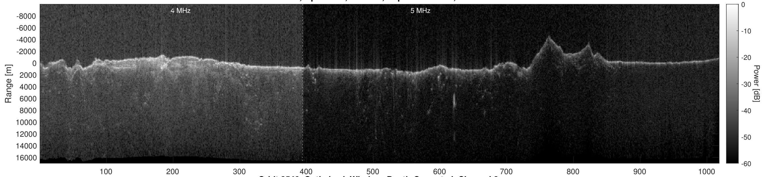
Orbit 8540, Optimized, Window, Depth-Corrected, Channel 2
