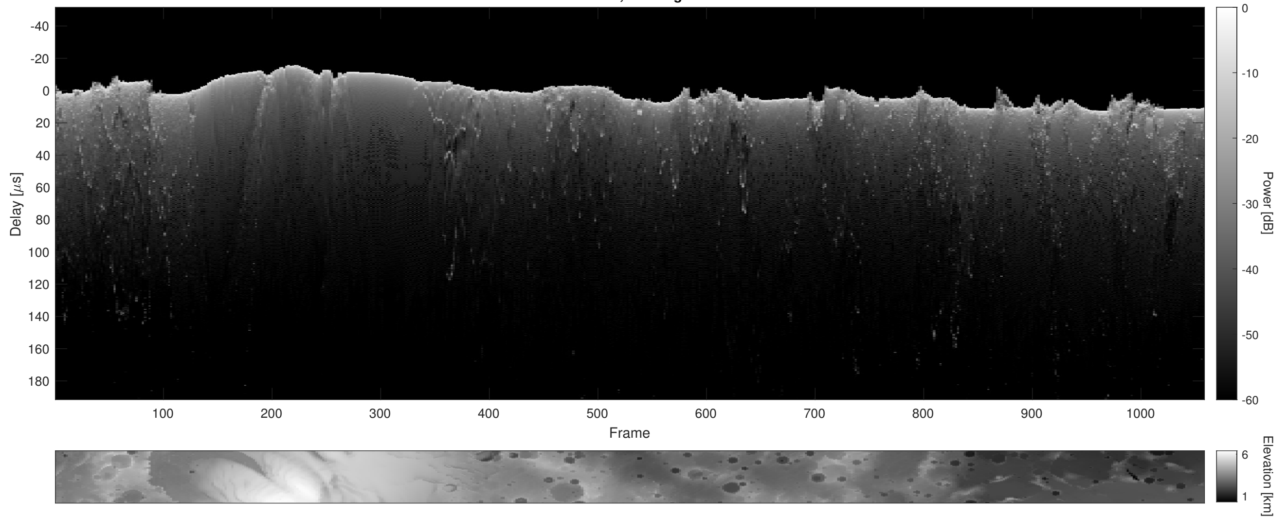
Orbit 8544, Cluttergram
