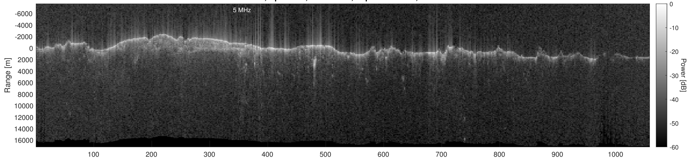
Orbit 8544, Optimized, No Window, Depth-Corrected, Channel 2
