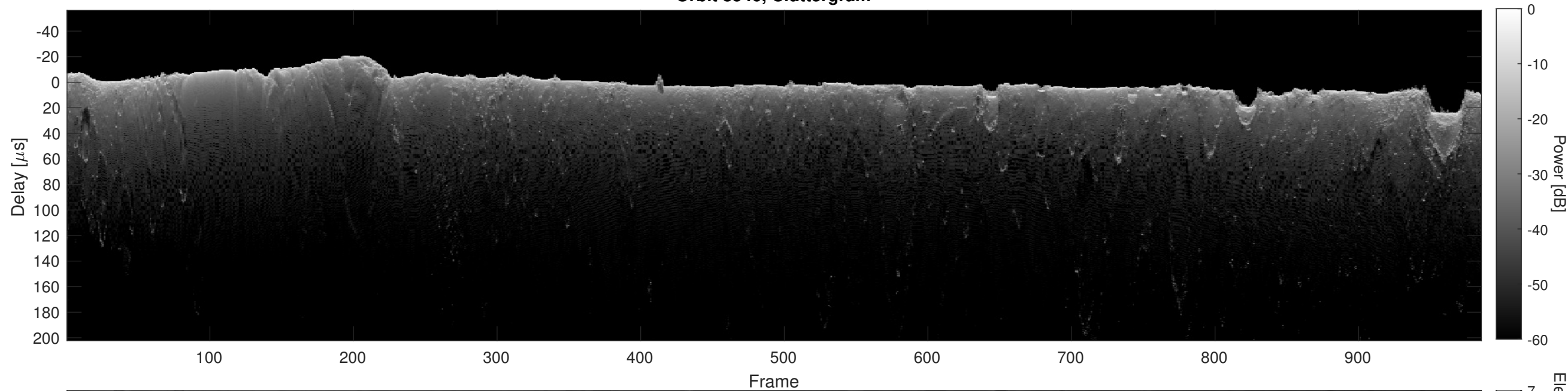
Orbit 8546, Cluttergram
