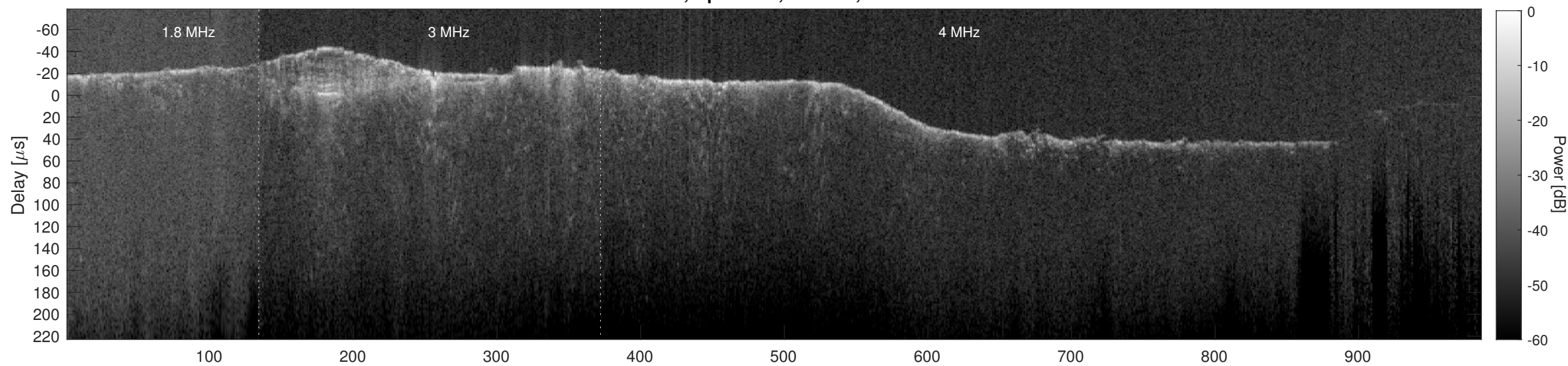
Orbit 8549, Cluttergram
