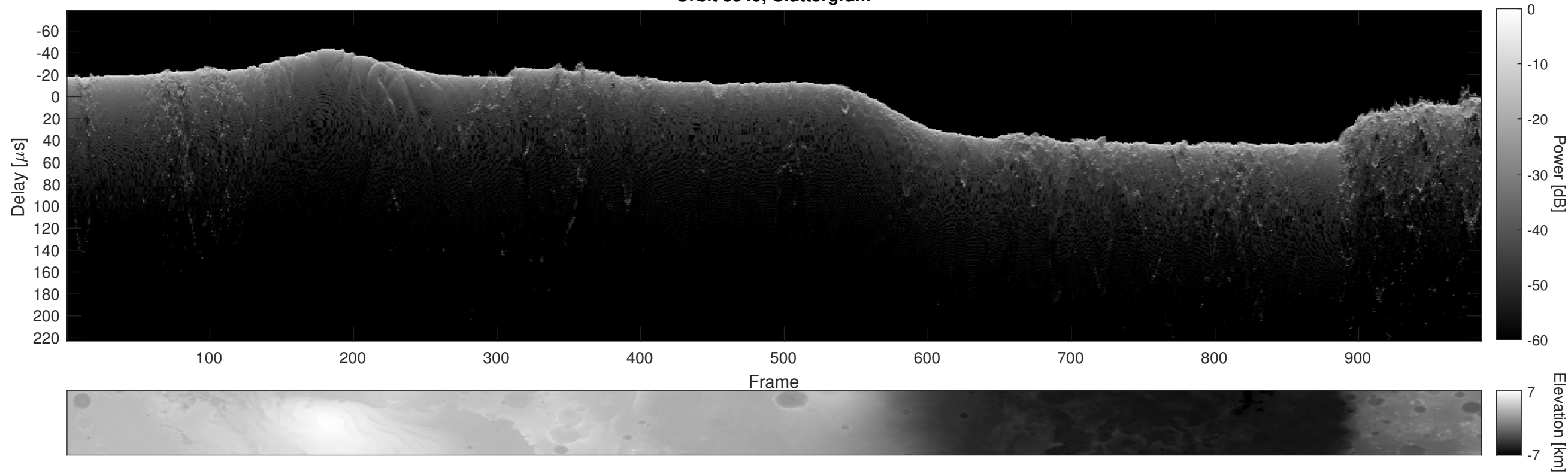
Orbit 8549, Cluttergram
