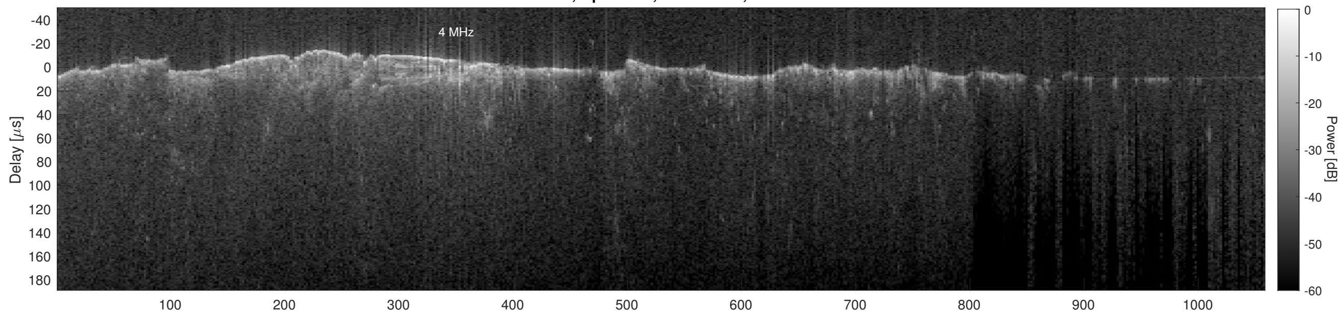
Orbit 8551, Cluttergram
