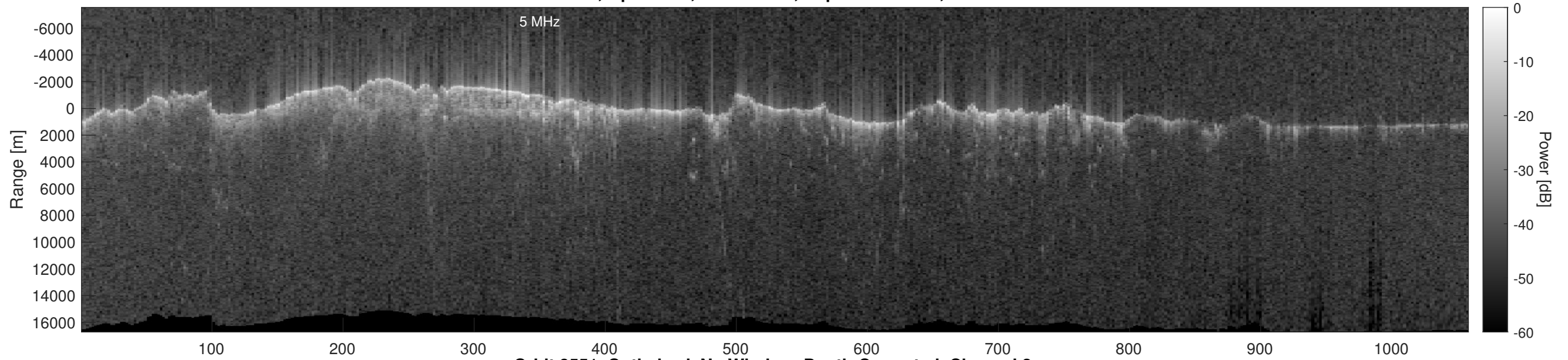
Orbit 8551, Optimized, No Window, Depth-Corrected, Channel 2
