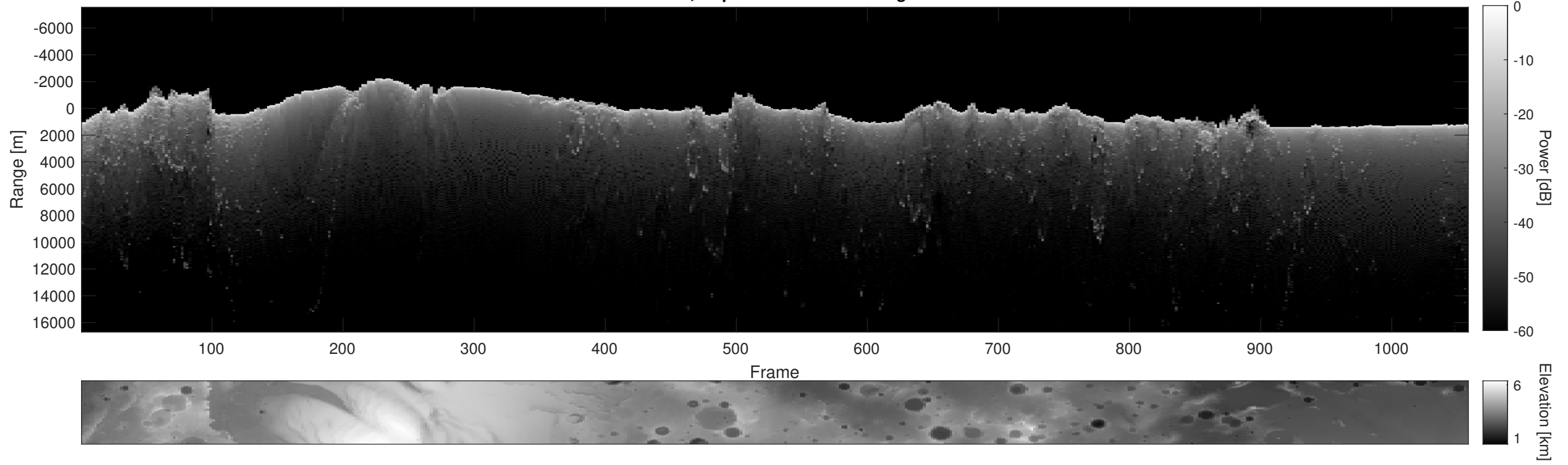
Orbit 8551, Depth-Corrected Cluttergram
