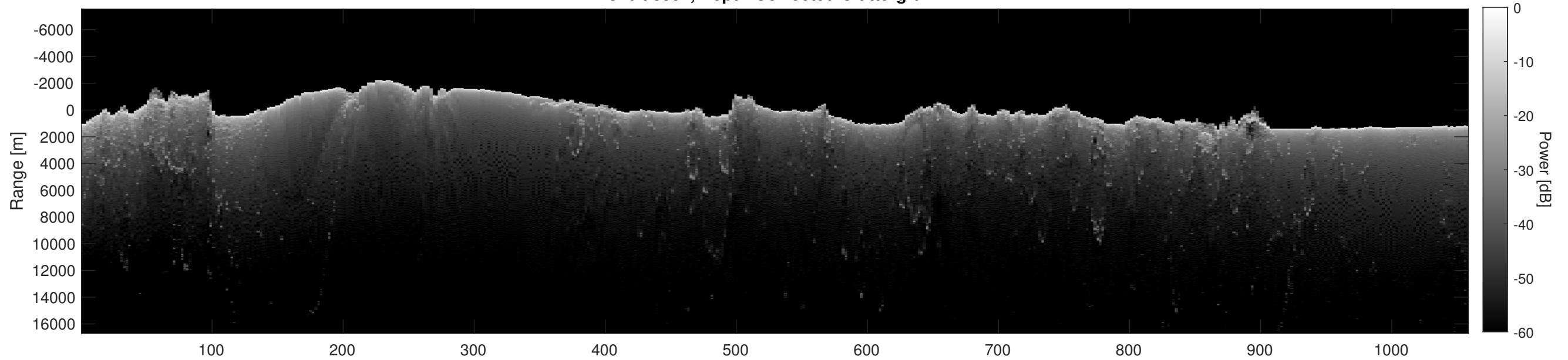
Orbit 8551, Depth-Corrected Cluttergram
