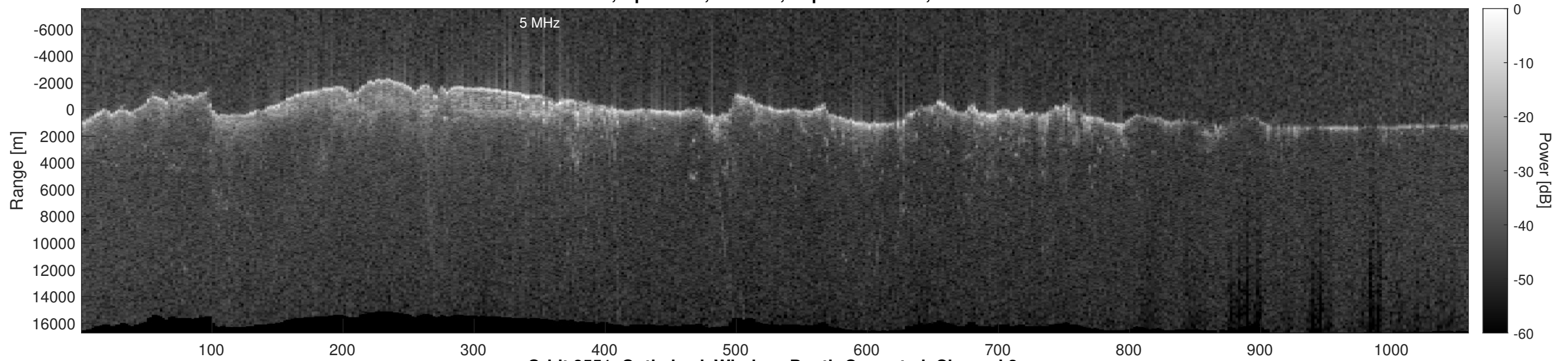
Orbit 8551, Optimized, Window, Depth-Corrected, Channel 2
