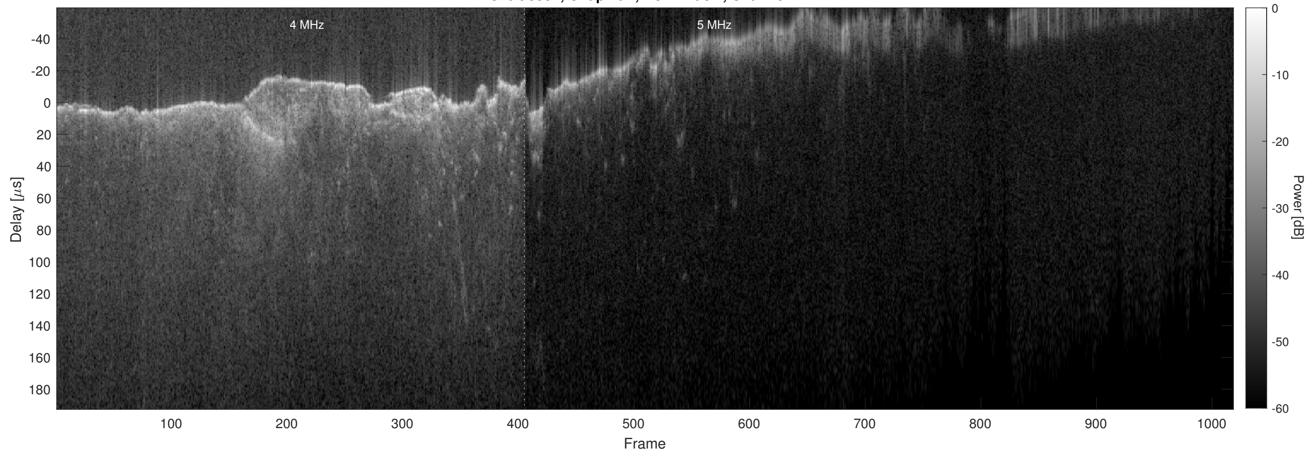
Orbit 8552, Chapman, No Window, Channel 2
