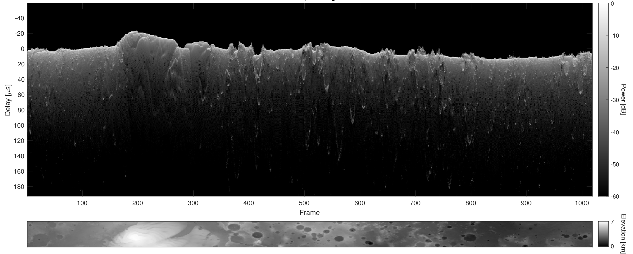
Orbit 8552, Cluttergram
