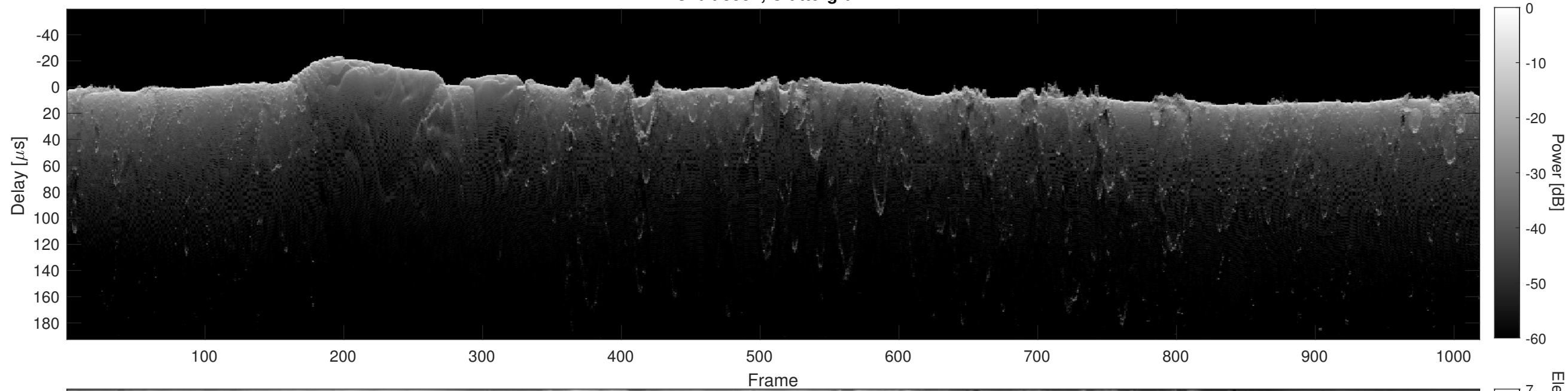
Orbit 8552, Cluttergram
