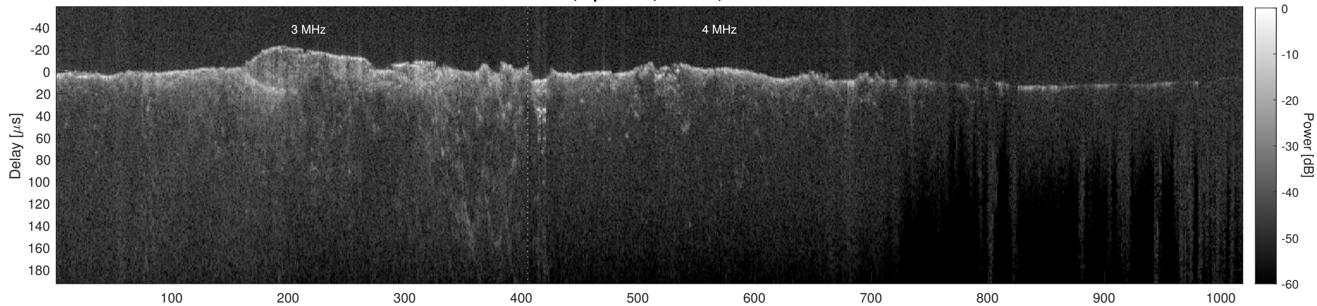
Orbit 8552, Cluttergram
