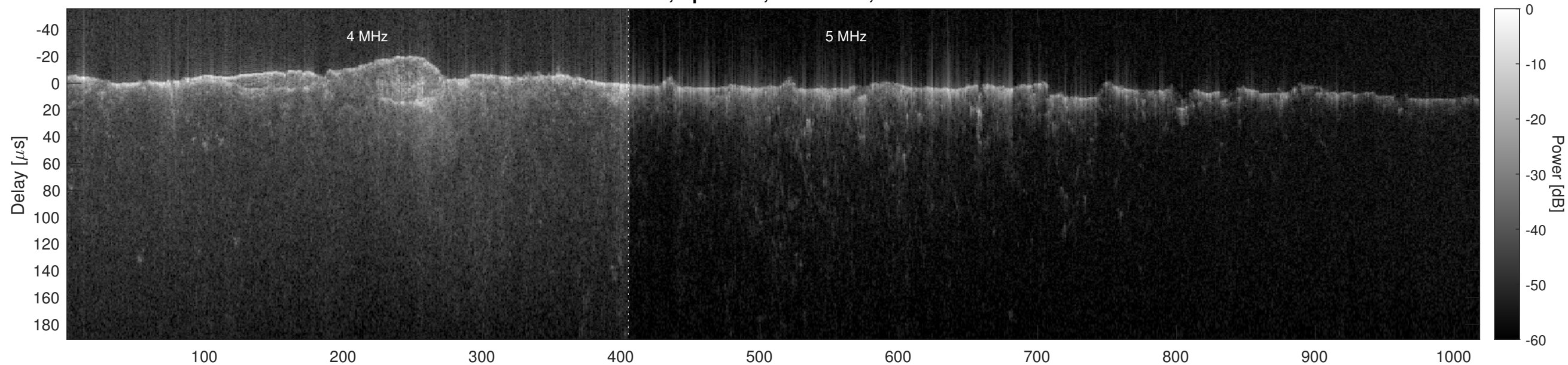
Orbit 8553, Optimized, No Window, Channel 2
