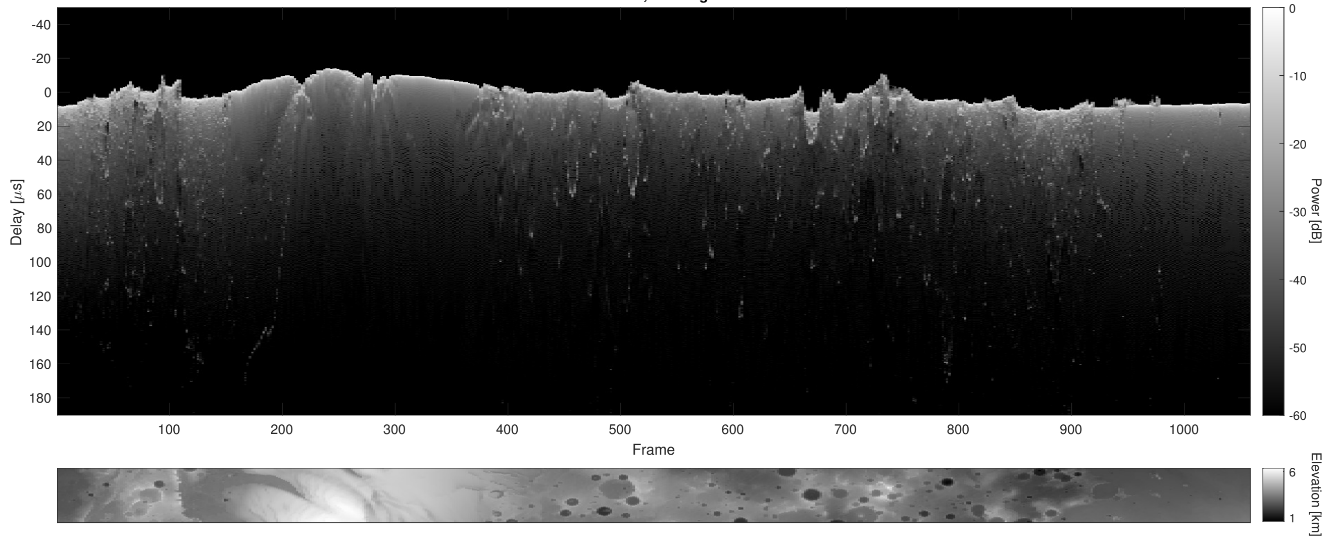
Orbit 8558, Cluttergram
