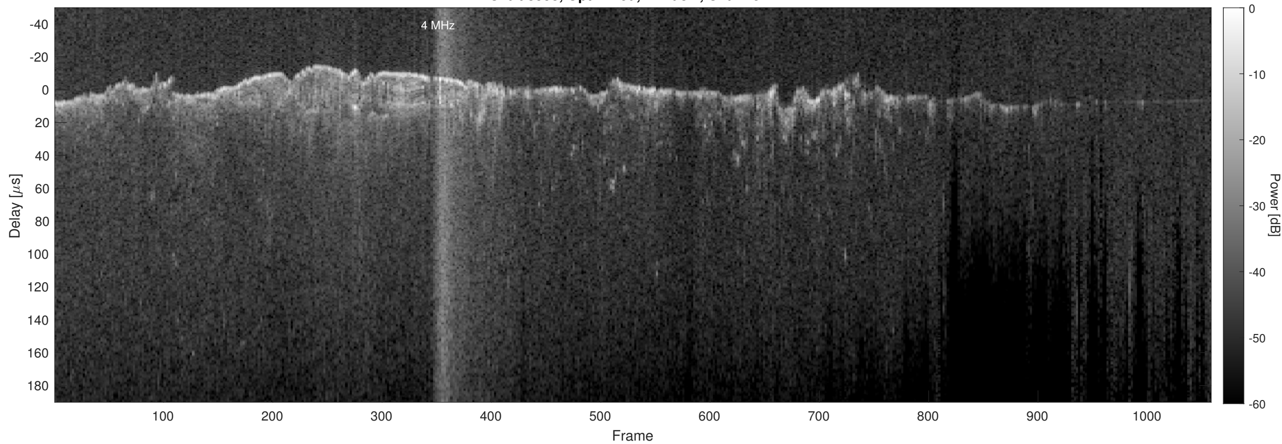
Orbit 8558, Optimized, Window, Channel 2
