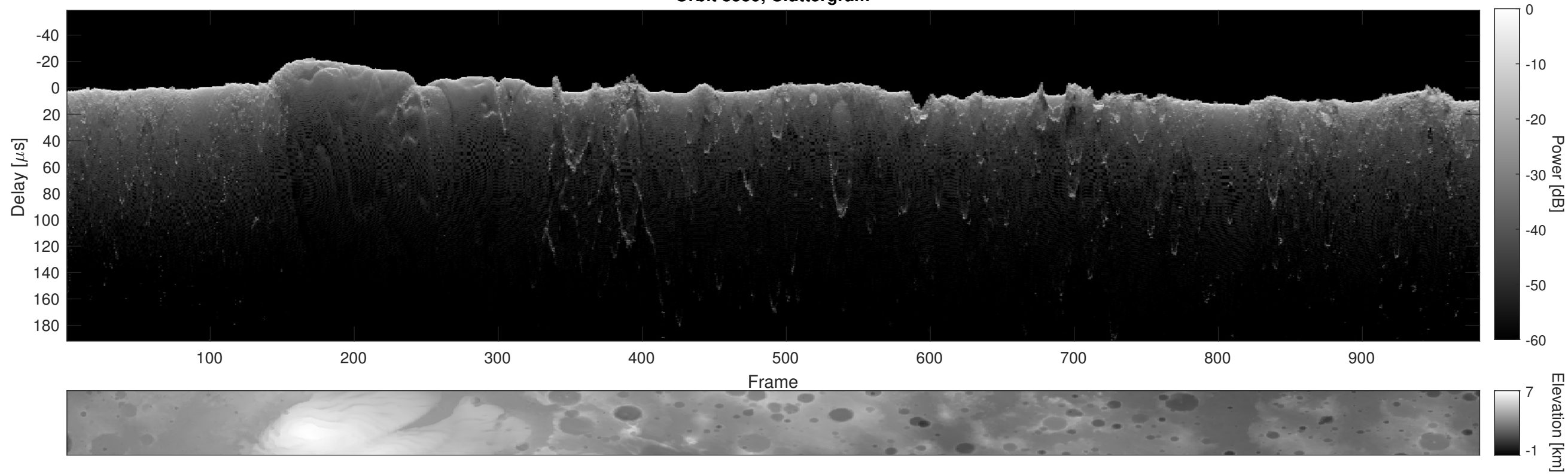
Orbit 8559, Cluttergram
