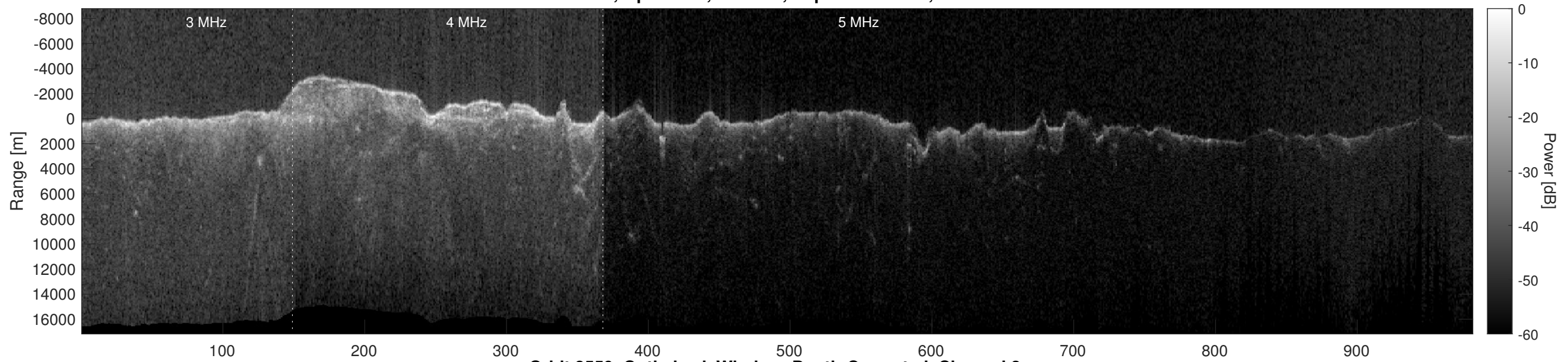
Orbit 8559, Optimized, Window, Depth-Corrected, Channel 2
