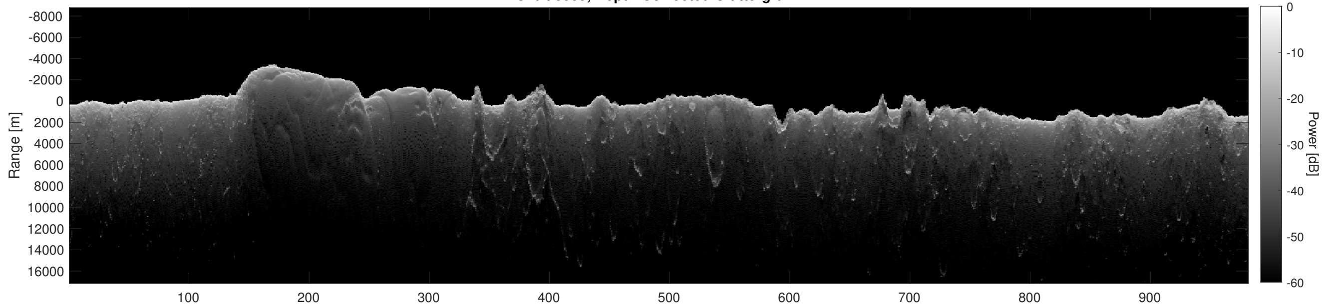
Orbit 8559, Depth-Corrected Cluttergram
