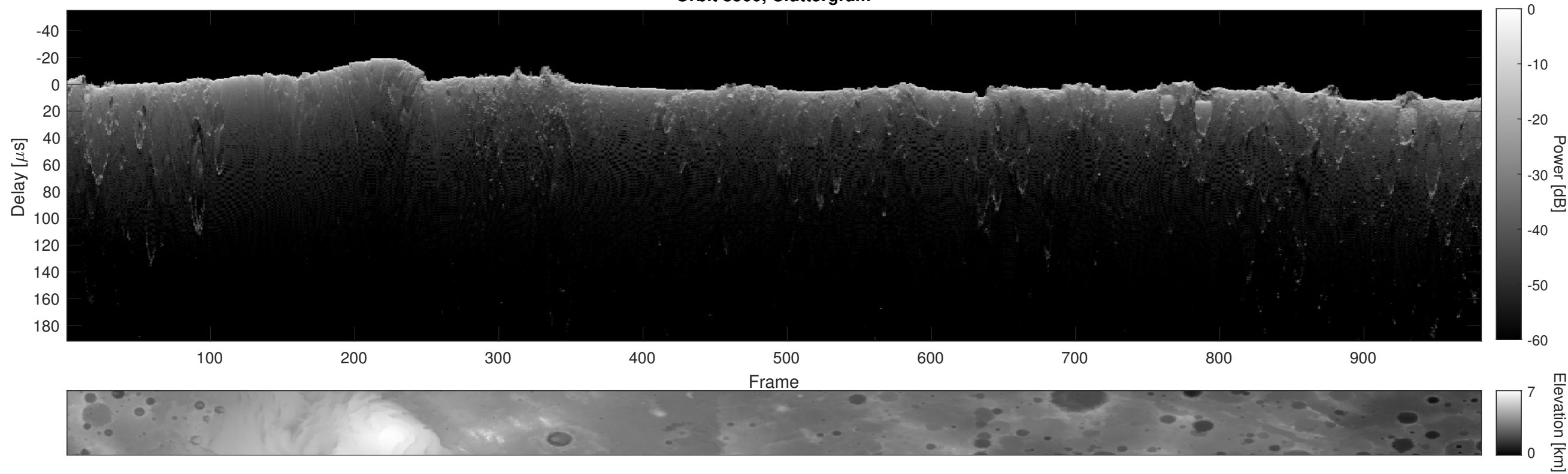
Orbit 8560, Cluttergram
