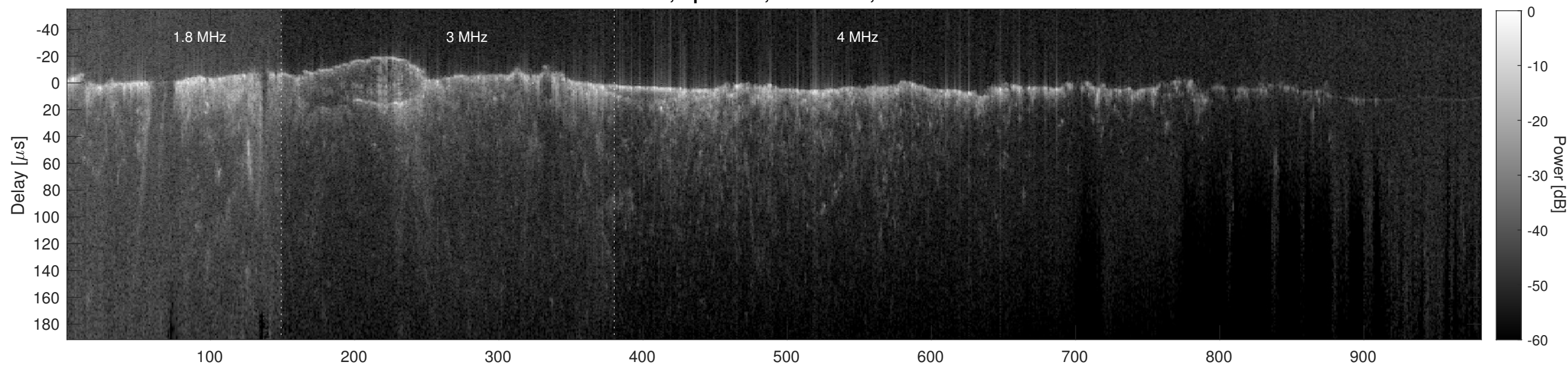
Orbit 8560, Cluttergram
