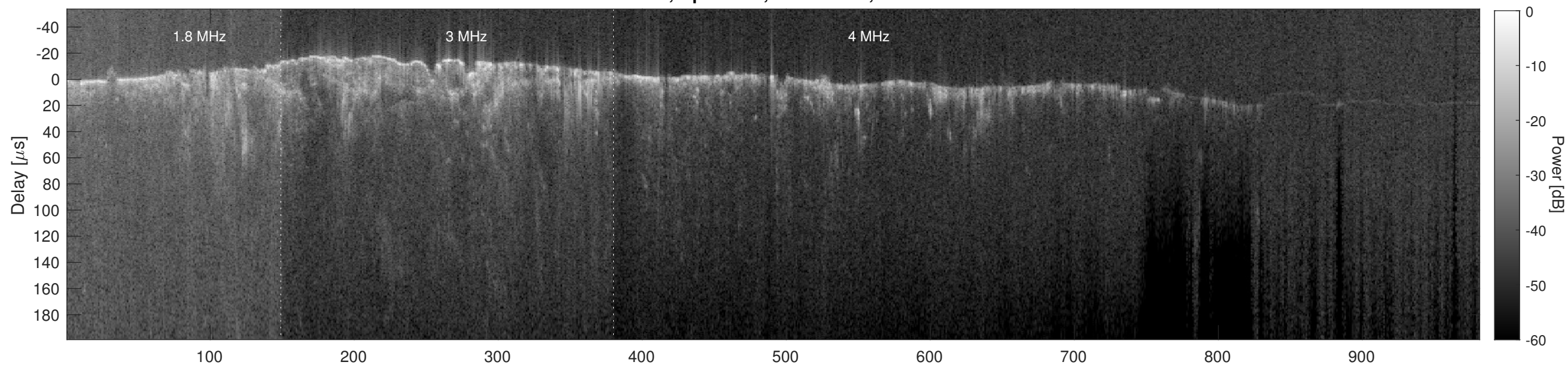
Orbit 8562, Cluttergram
