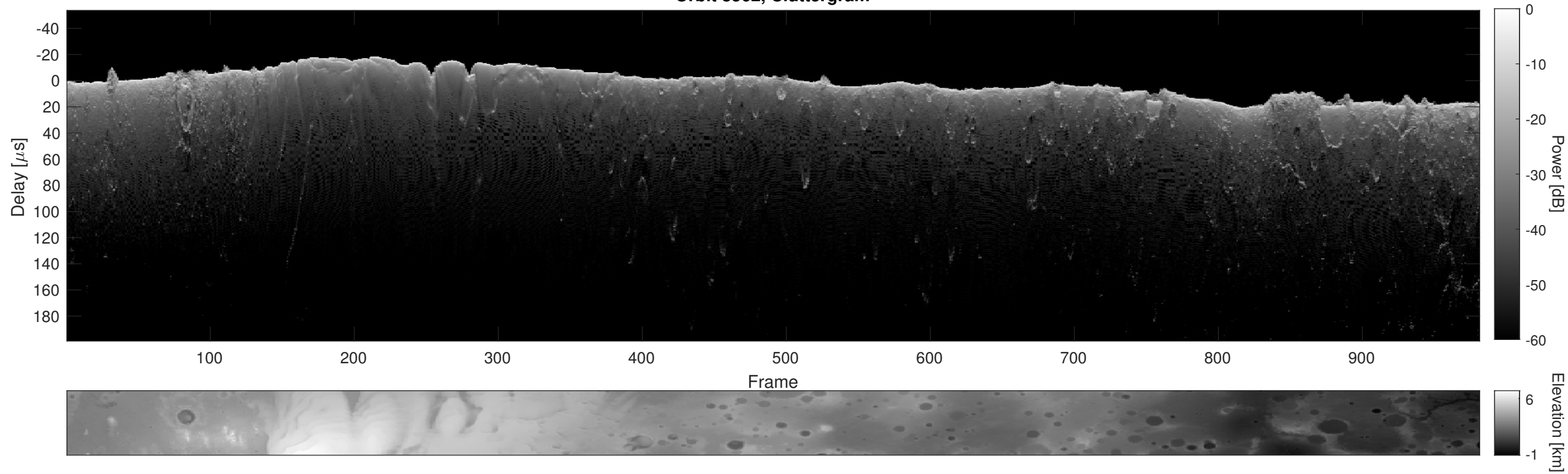
Orbit 8562, Cluttergram
