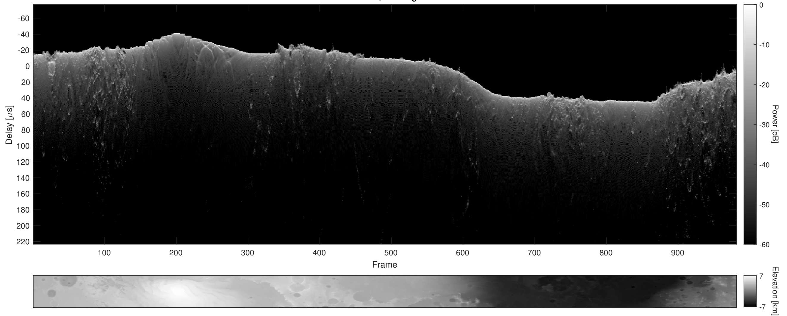
Orbit 8563, Cluttergram
