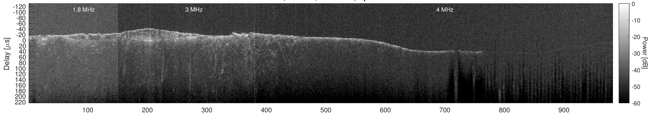
Orbit 8563, Cluttergram
