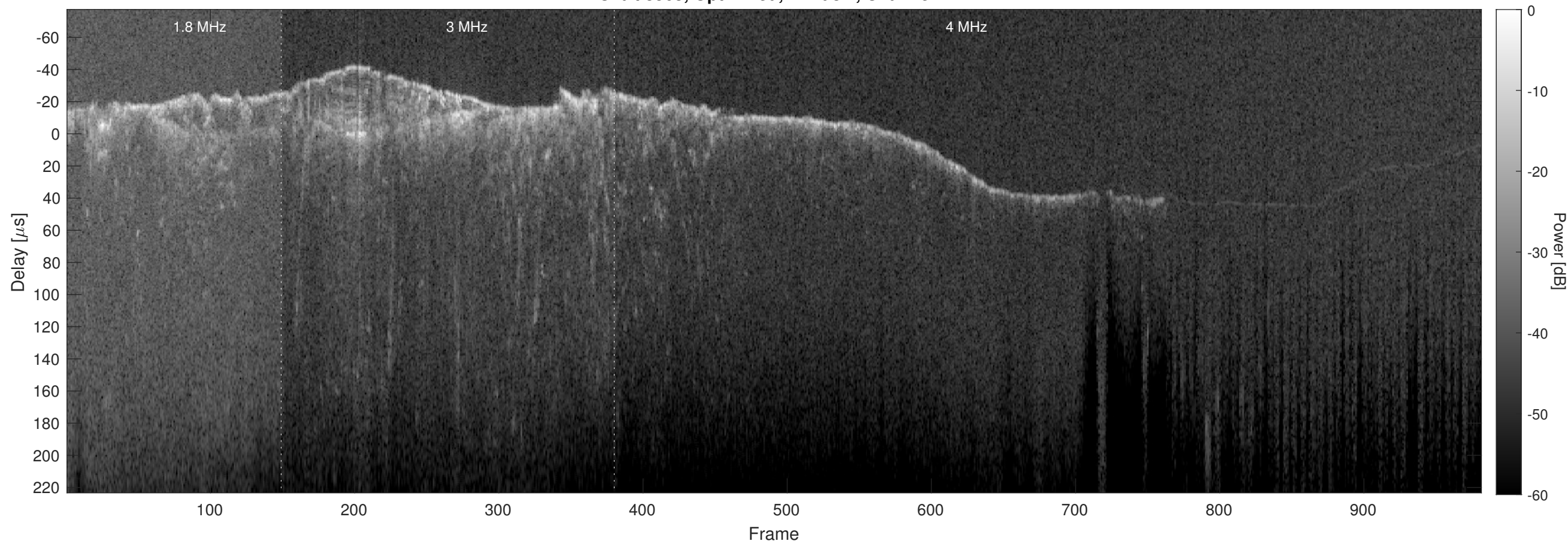
Orbit 8563, Optimized, Window, Channel 2
