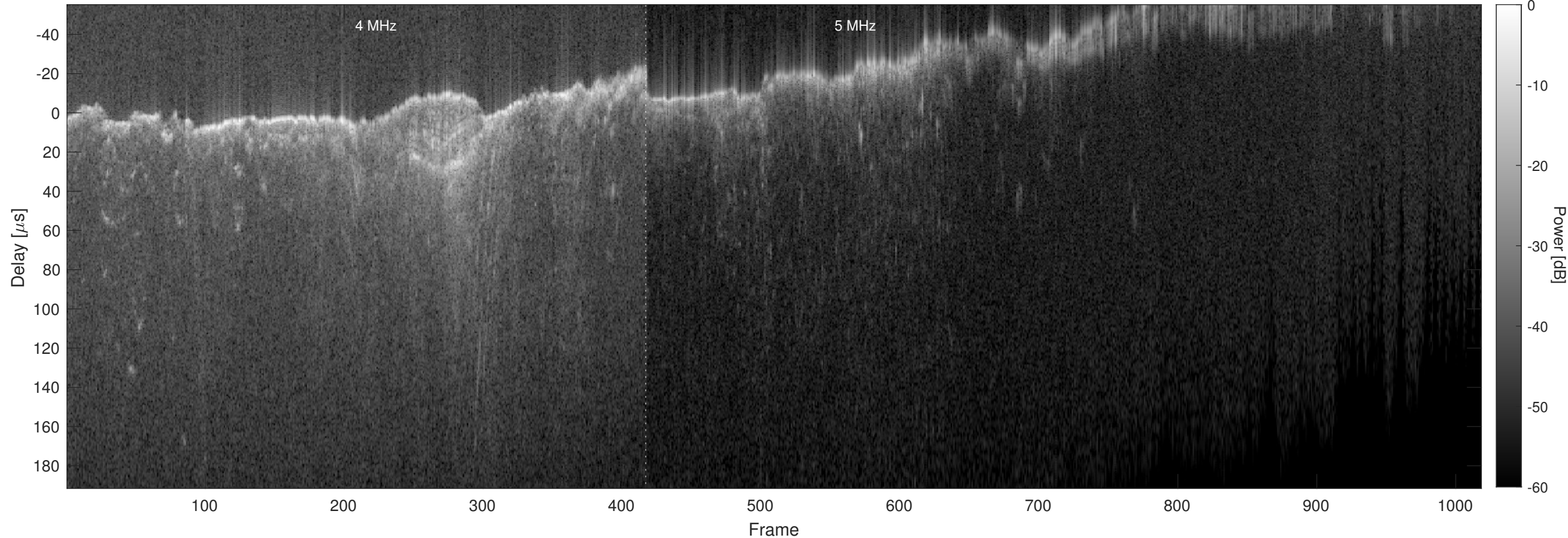
Orbit 8567, Chapman, No Window, Channel 2
