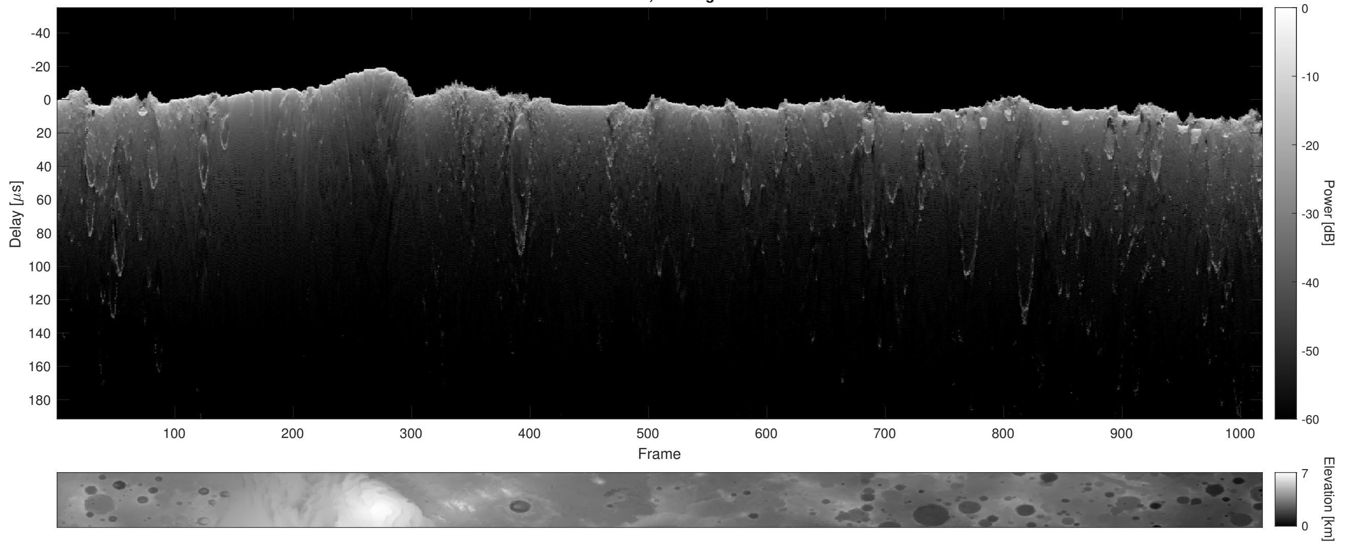
Orbit 8567, Cluttergram
