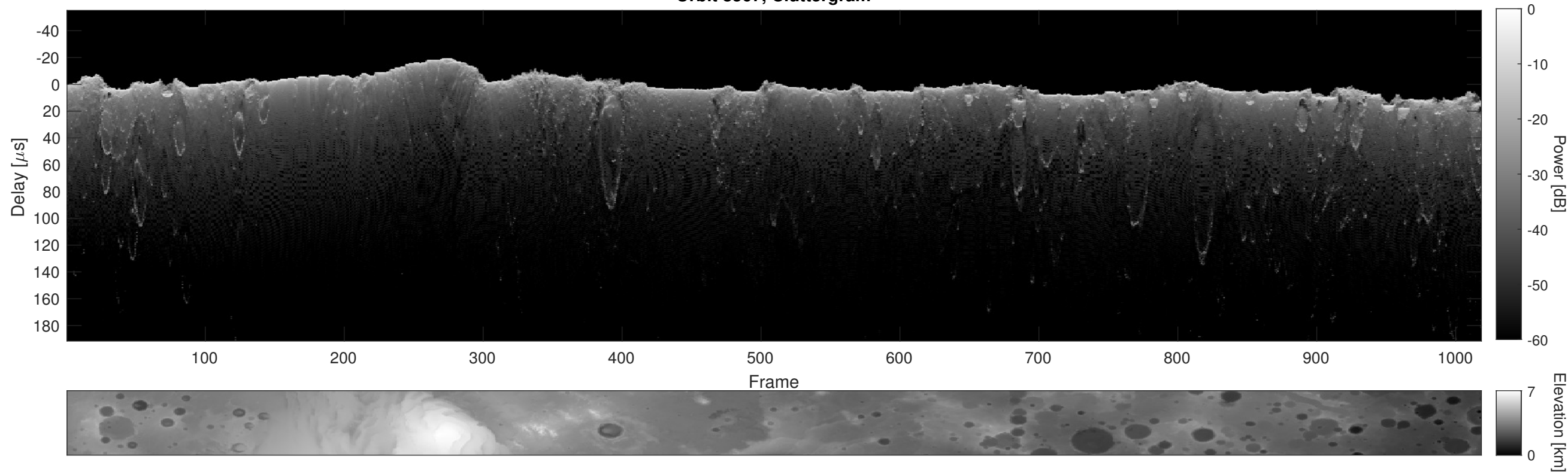
Orbit 8567, Cluttergram
