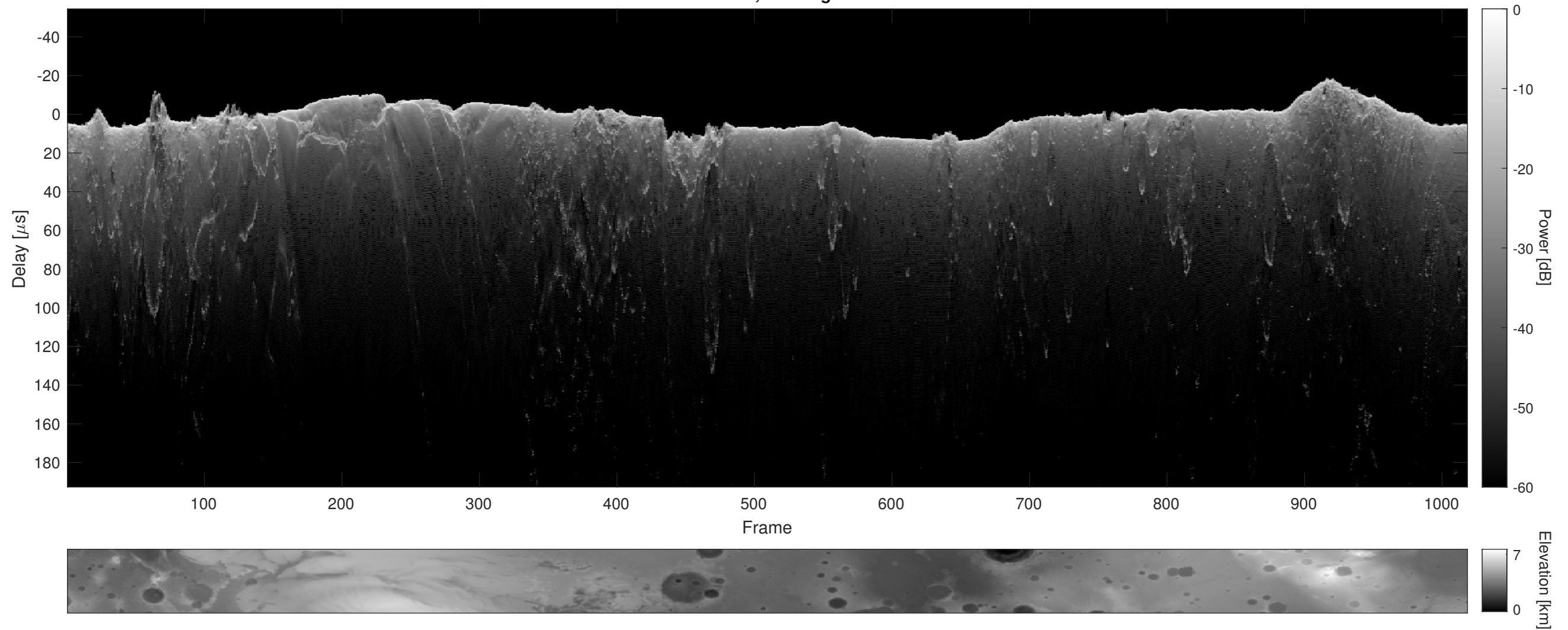
Orbit 8568, Cluttergram
