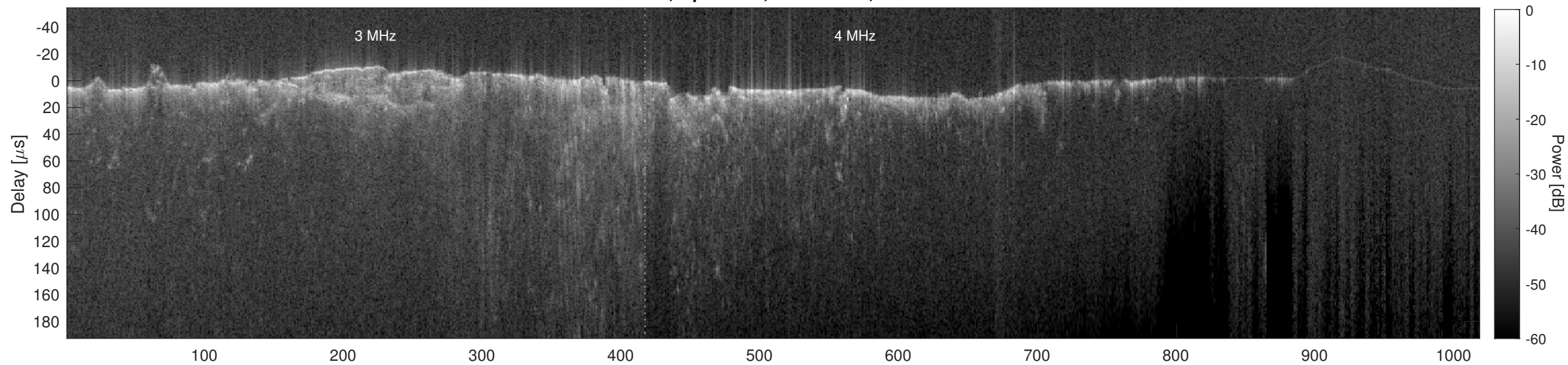
Orbit 8568, Cluttergram
