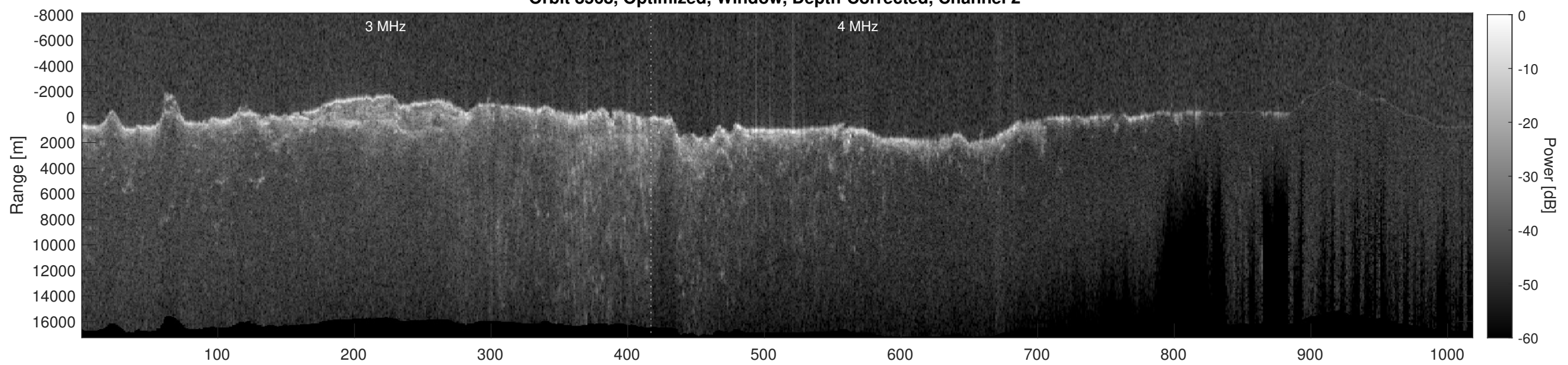
Orbit 8568, Depth-Corrected Cluttergram
