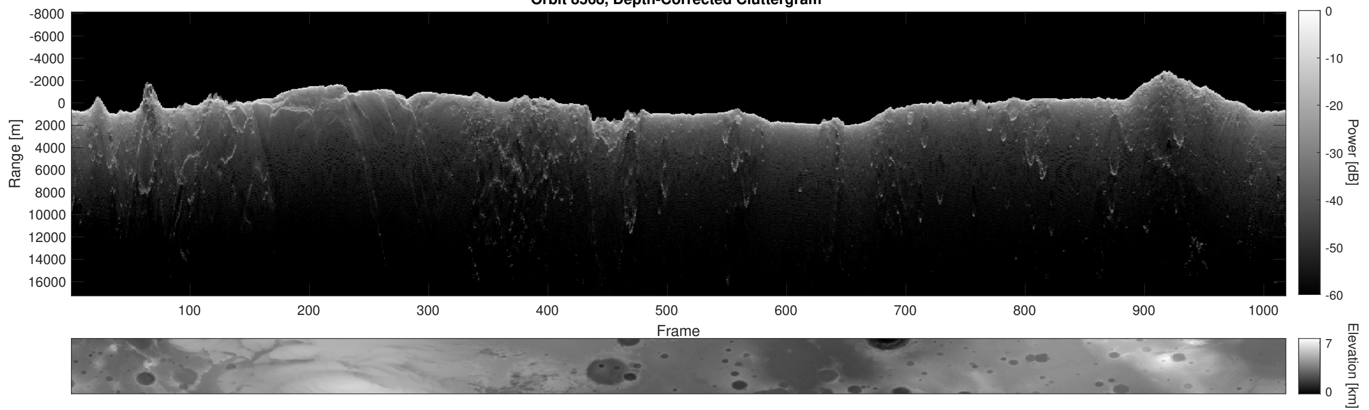
Orbit 8568, Depth-Corrected Cluttergram
