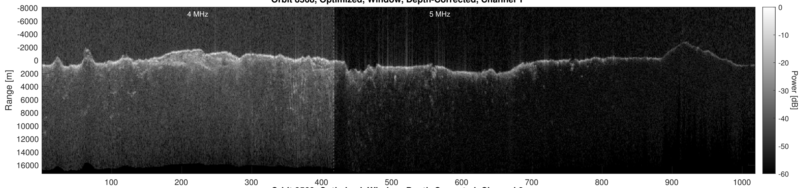
Orbit 8568, Optimized, Window, Depth-Corrected, Channel 2
