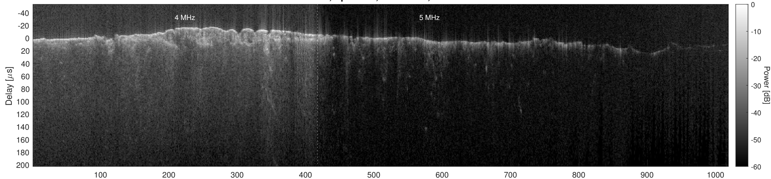
Orbit 8569, Optimized, No Window, Channel 2
