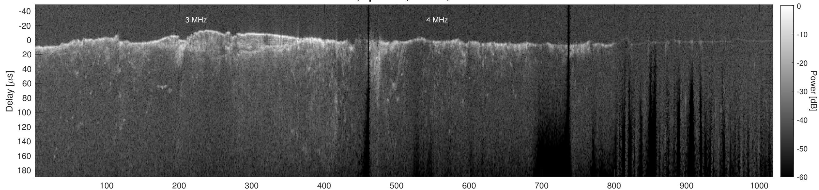
Orbit 8572, Cluttergram
