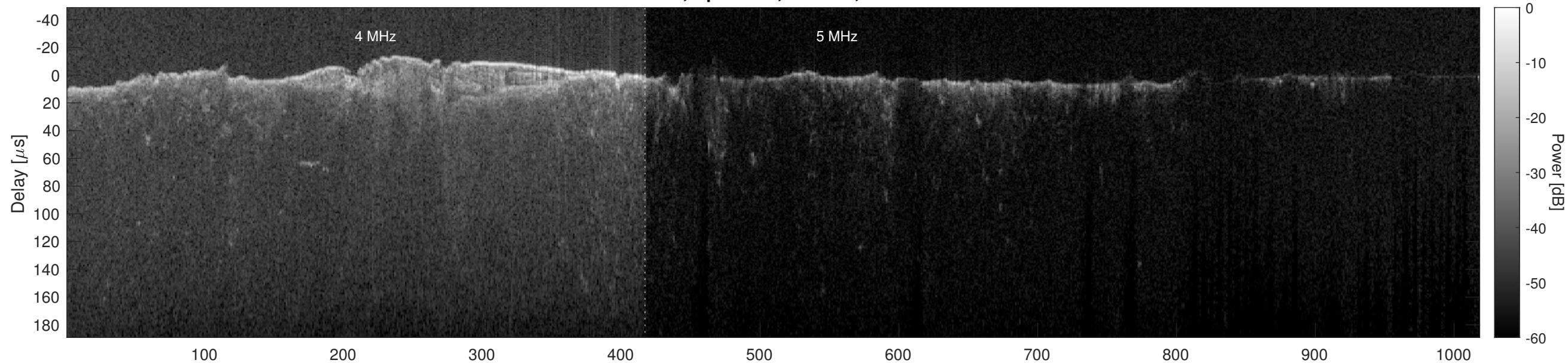
Orbit 8572, Optimized, Window, Channel 2
