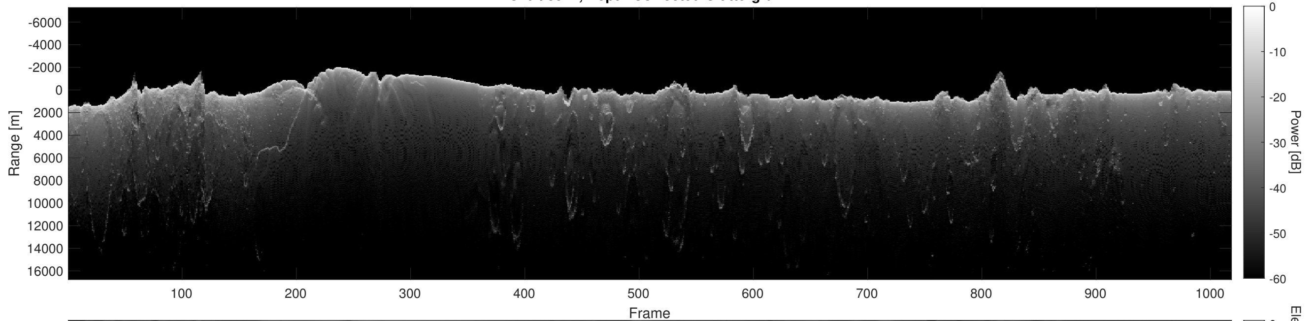
Orbit 8572, Depth-Corrected Cluttergram
