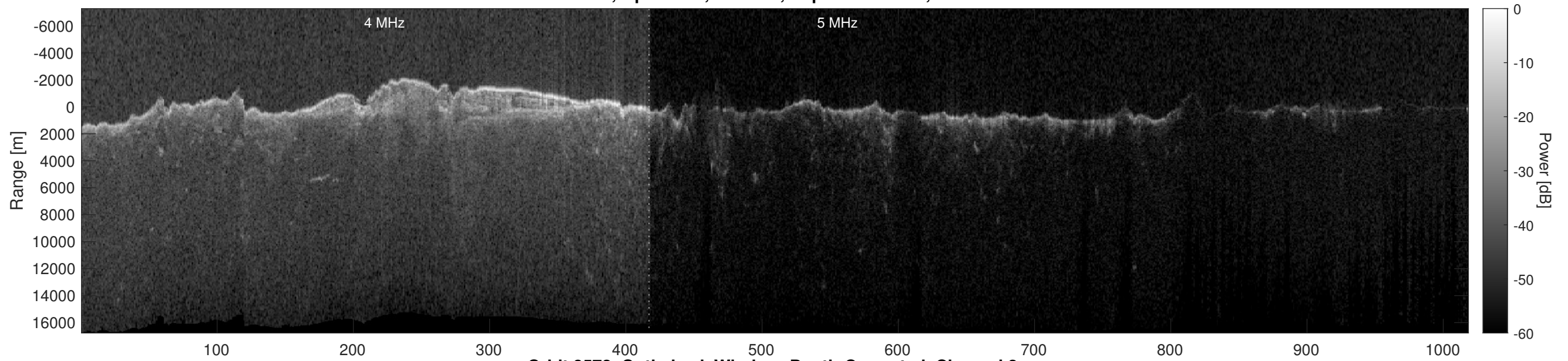
Orbit 8572, Optimized, Window, Depth-Corrected, Channel 2
