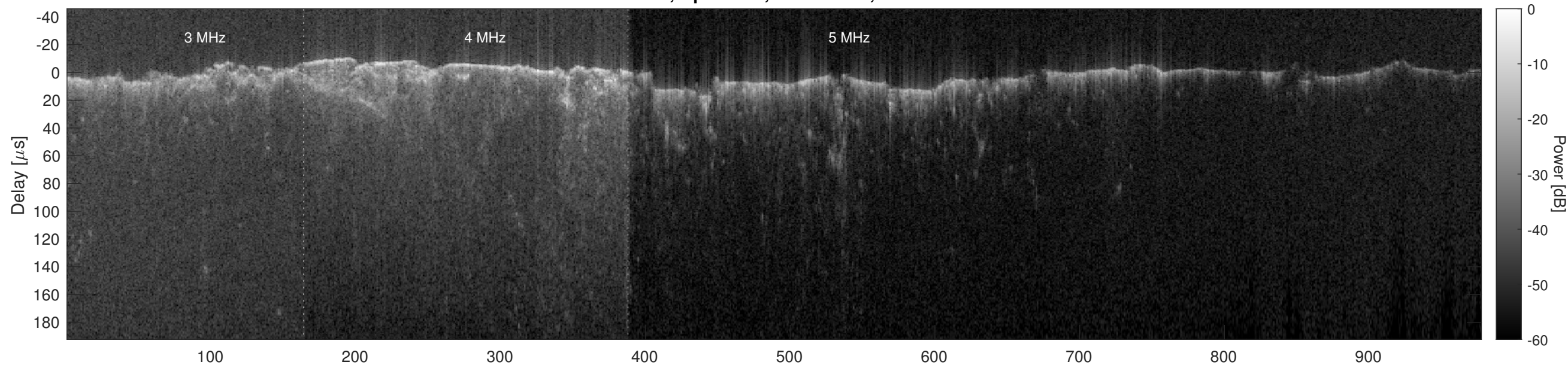
Orbit 8575, Optimized, No Window, Channel 2
