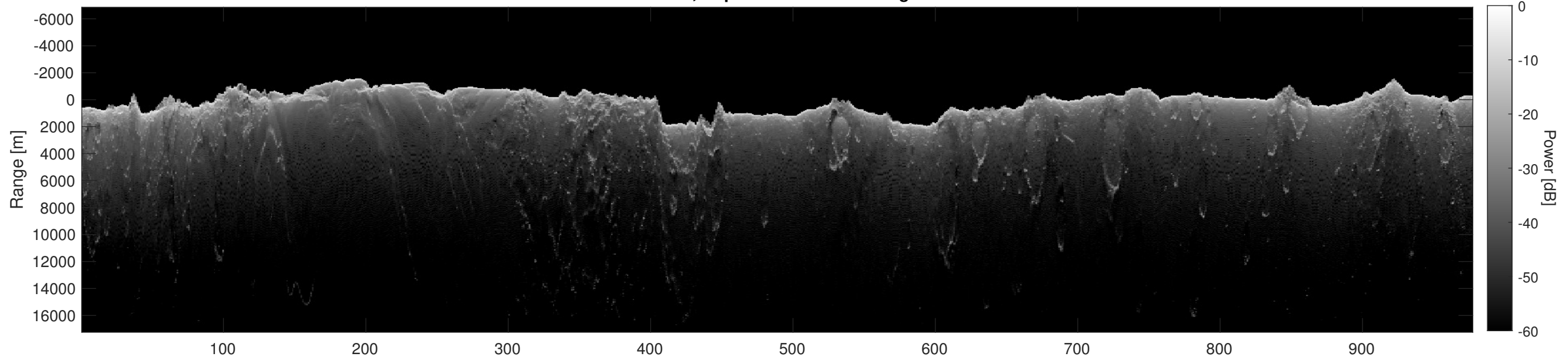
Orbit 8575, Depth-Corrected Cluttergram
