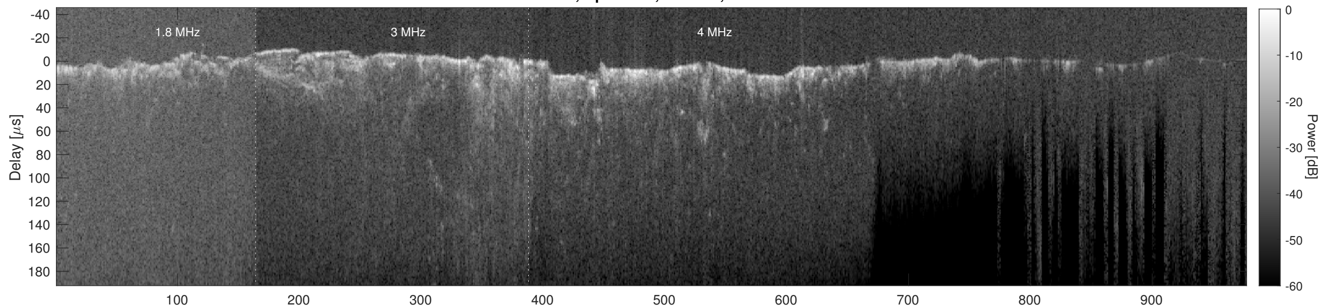
Orbit 8575, Cluttergram
