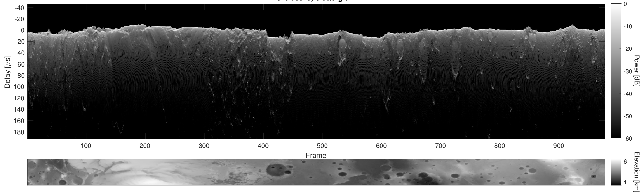
Orbit 8575, Cluttergram
