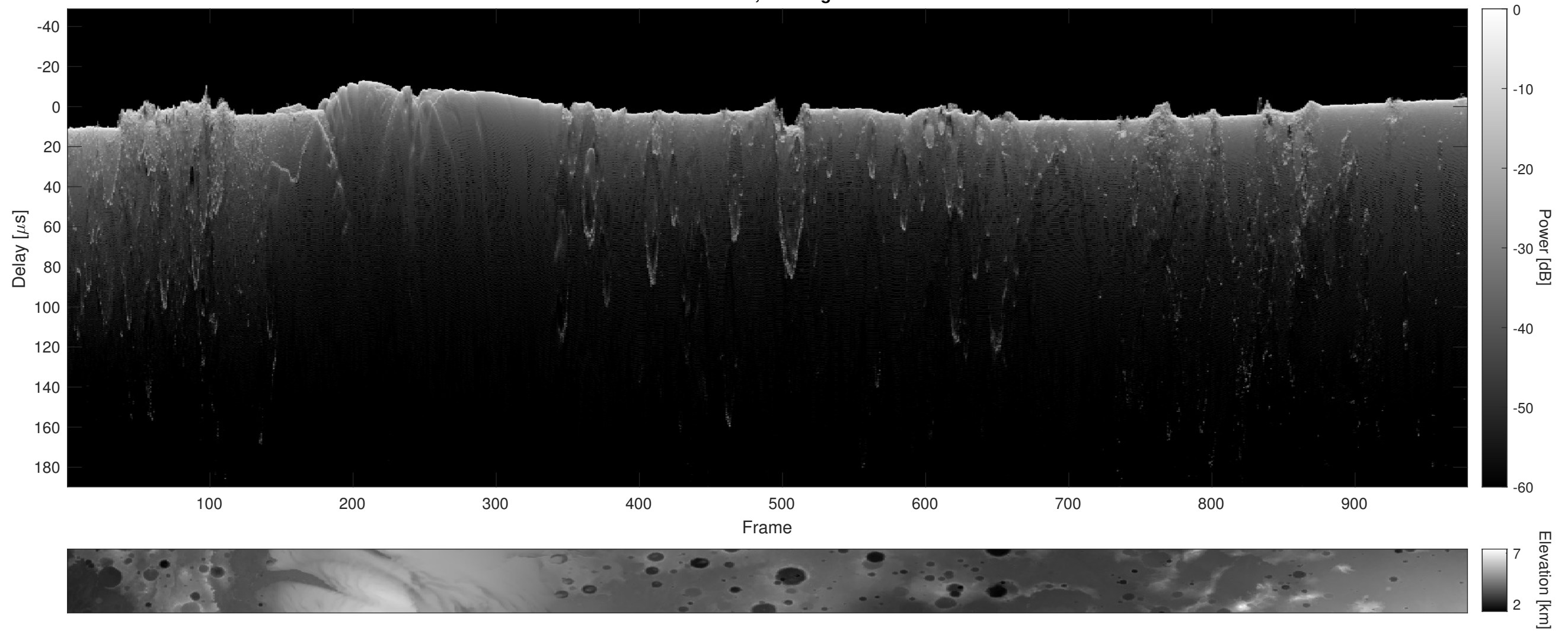
Orbit 8579, Cluttergram
