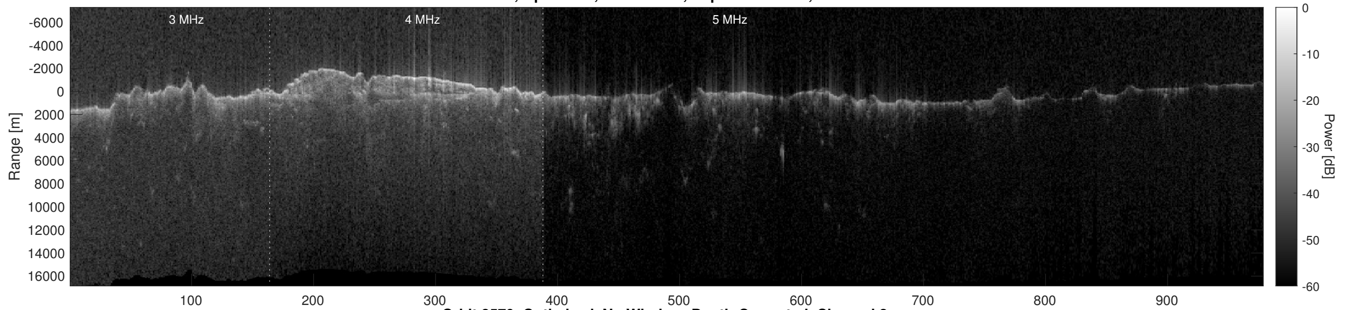
Orbit 8579, Optimized, No Window, Depth-Corrected, Channel 2
