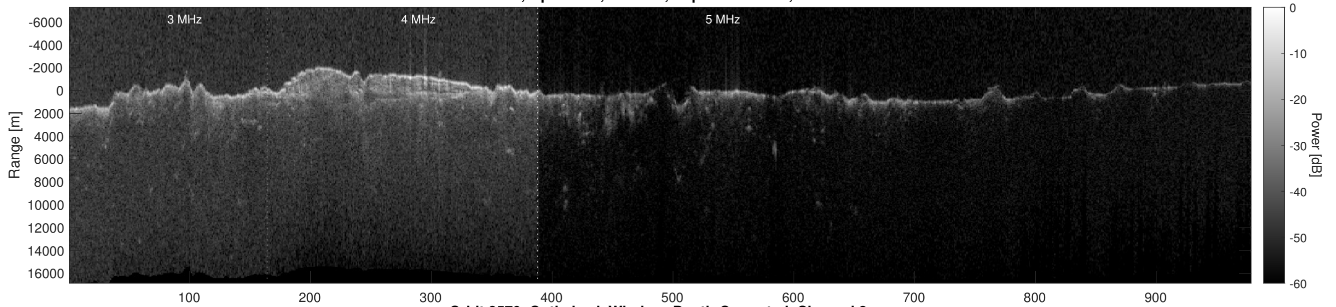
Orbit 8579, Optimized, Window, Depth-Corrected, Channel 2
