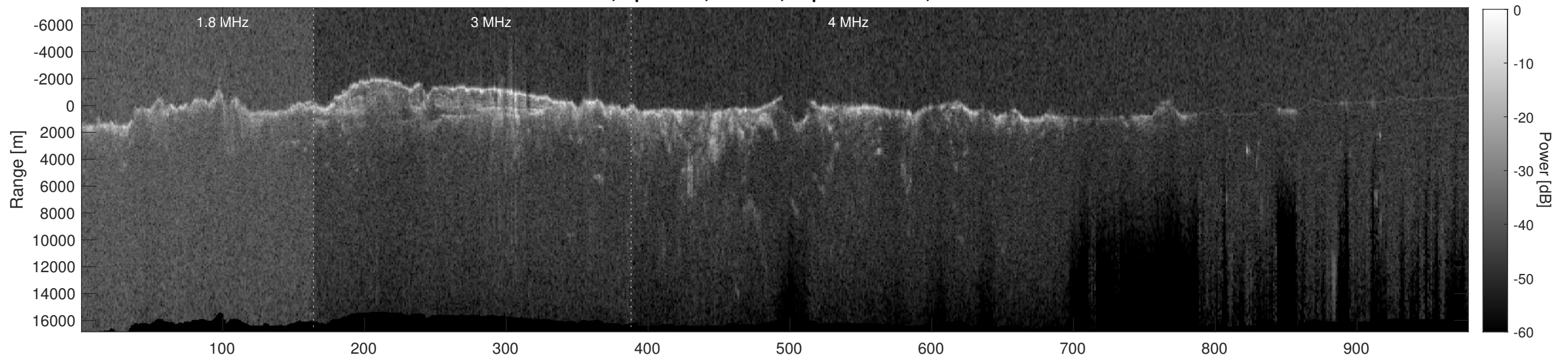
Orbit 8579, Depth-Corrected Cluttergram
