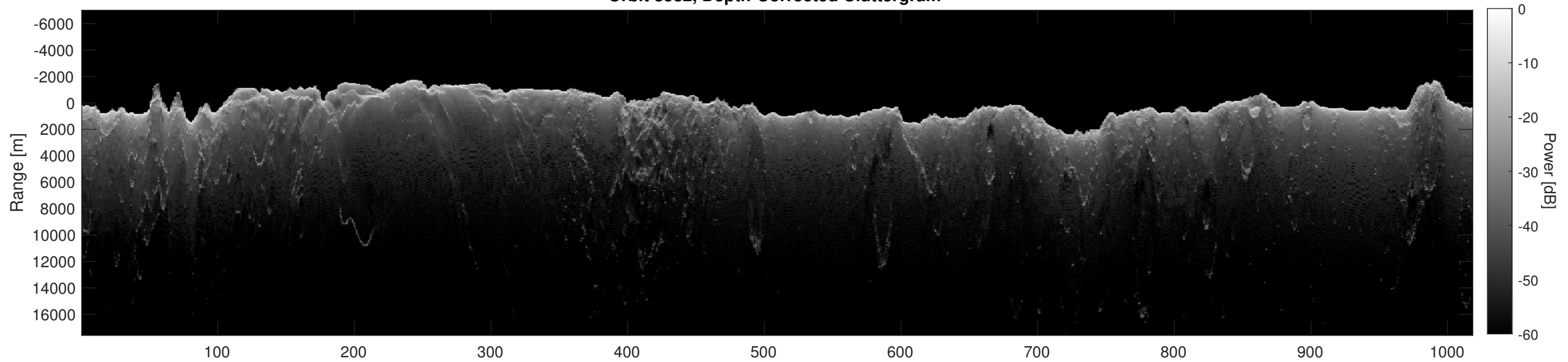
Orbit 8582, Depth-Corrected Cluttergram
