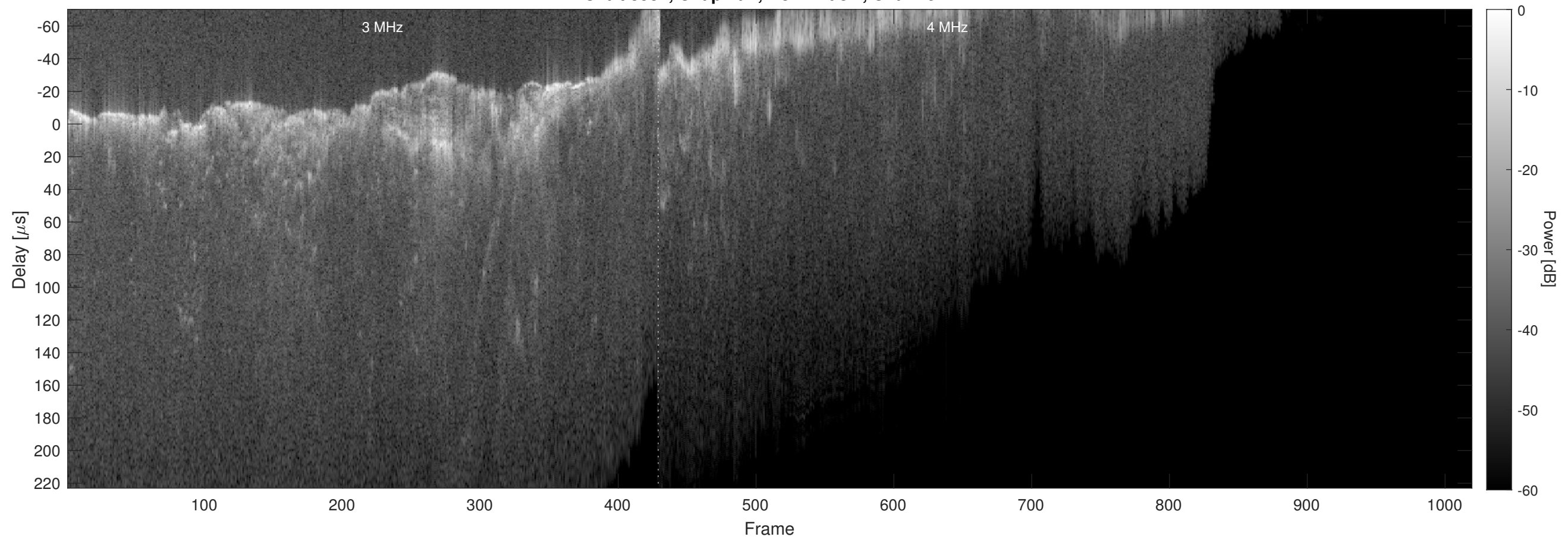
Orbit 8584, Chapman, No Window, Channel 2
