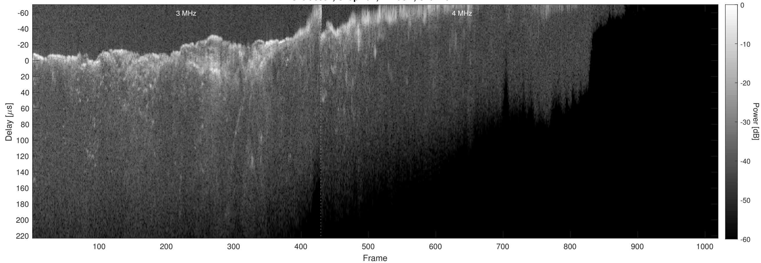
Orbit 8584, Chapman, Window, Channel 2
