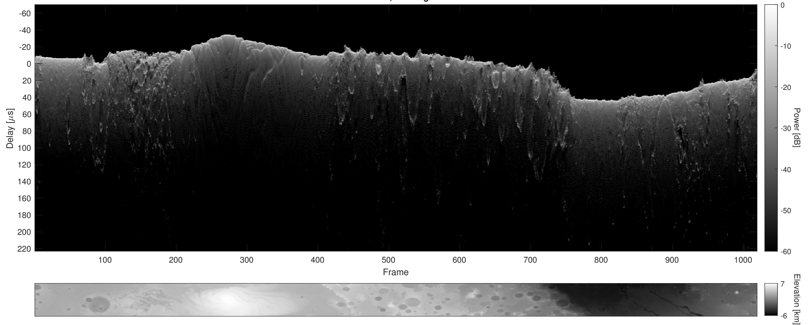
Orbit 8584, Cluttergram
