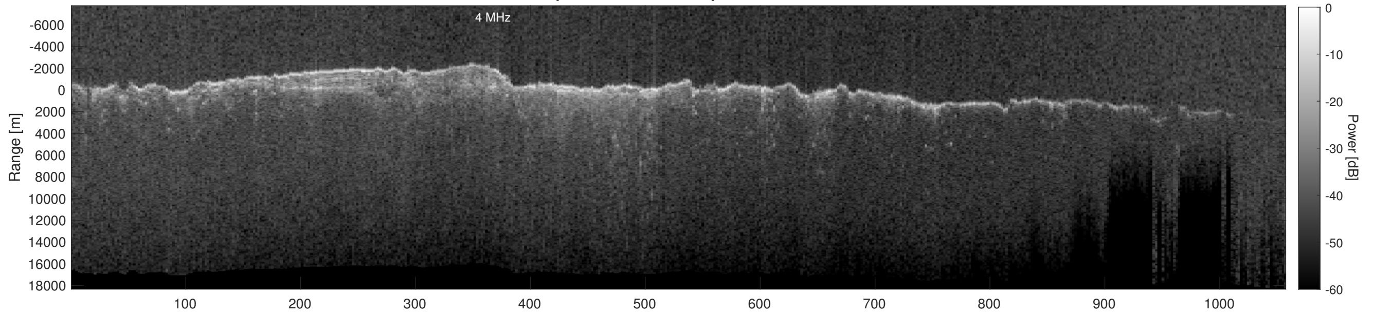
Orbit 8585, Depth-Corrected Cluttergram
