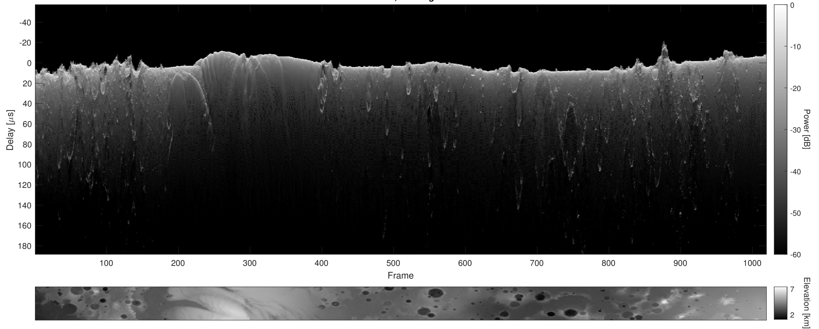
Orbit 8586, Cluttergram
