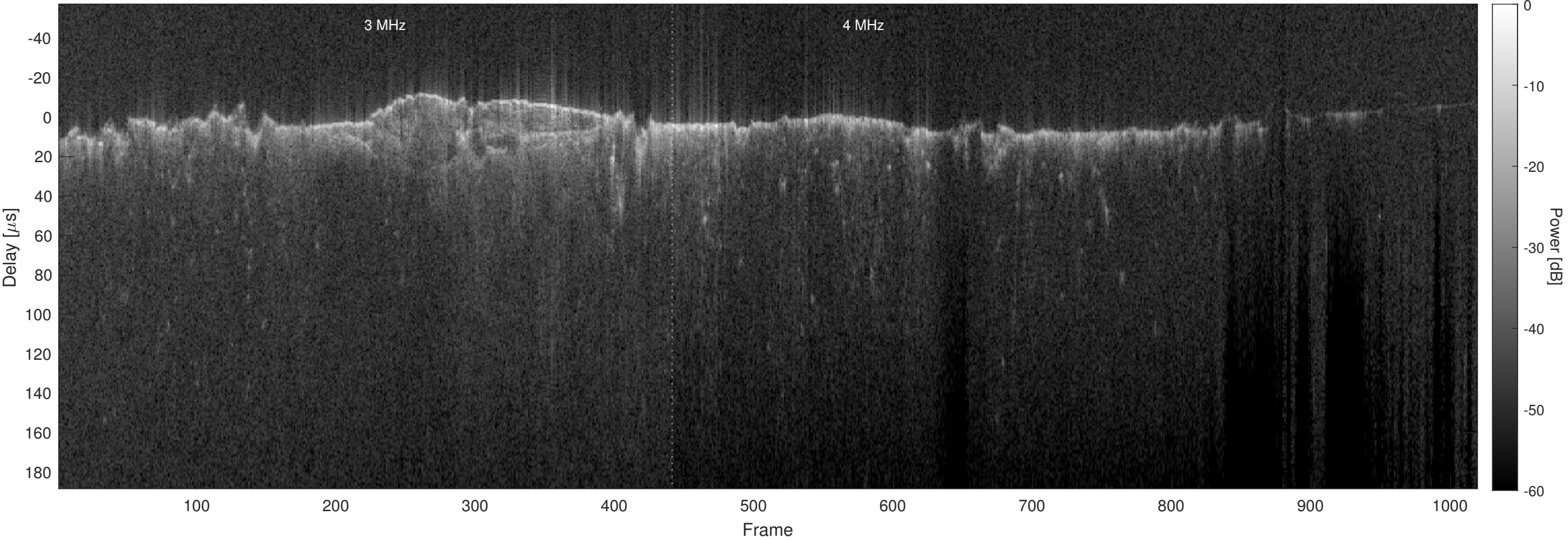
Orbit 8586, Optimized, No Window, Channel 2
