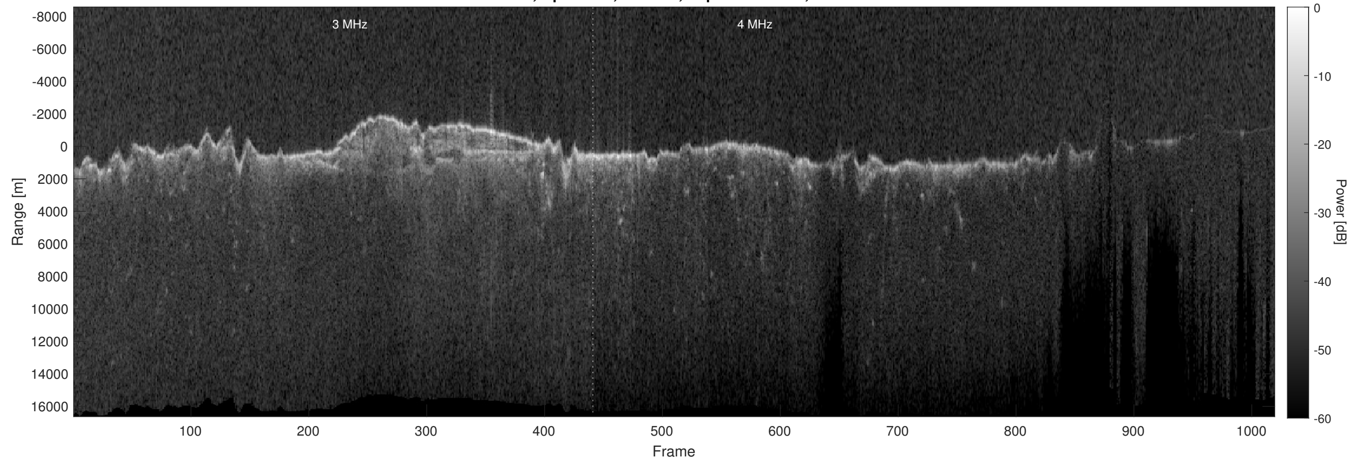
Orbit 8586, Optimized, Window, Depth-Corrected, Channel 2
