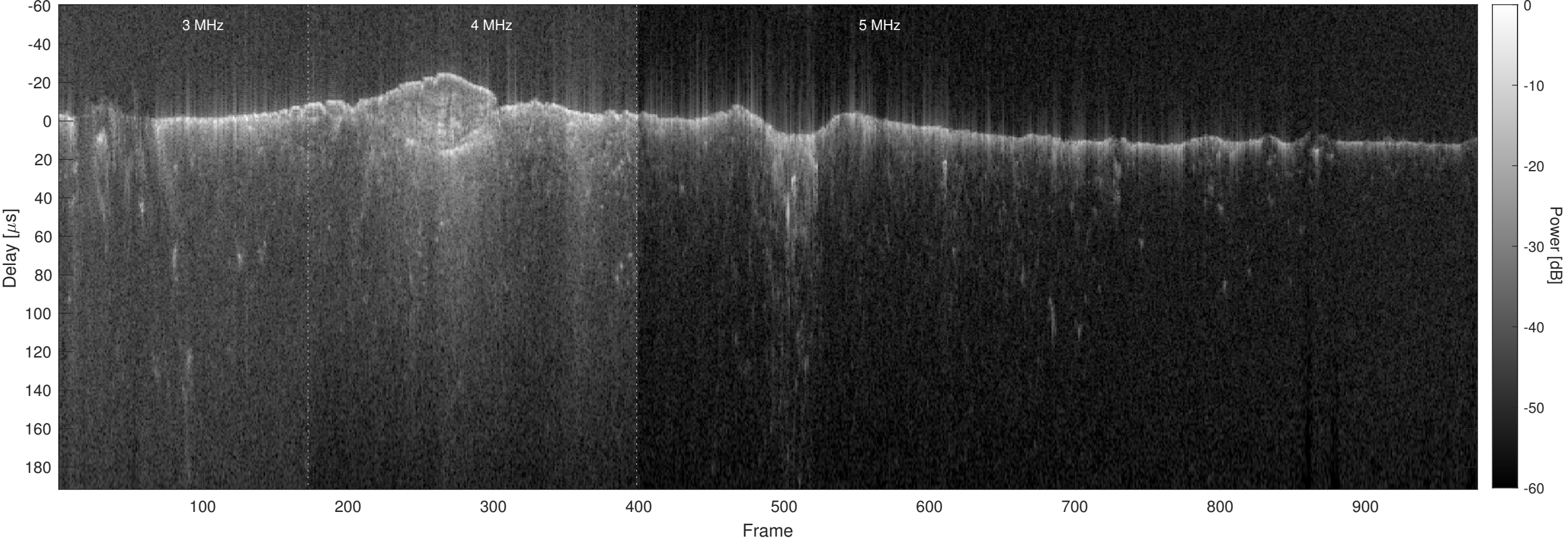
Orbit 8588, Optimized, No Window, Channel 2
