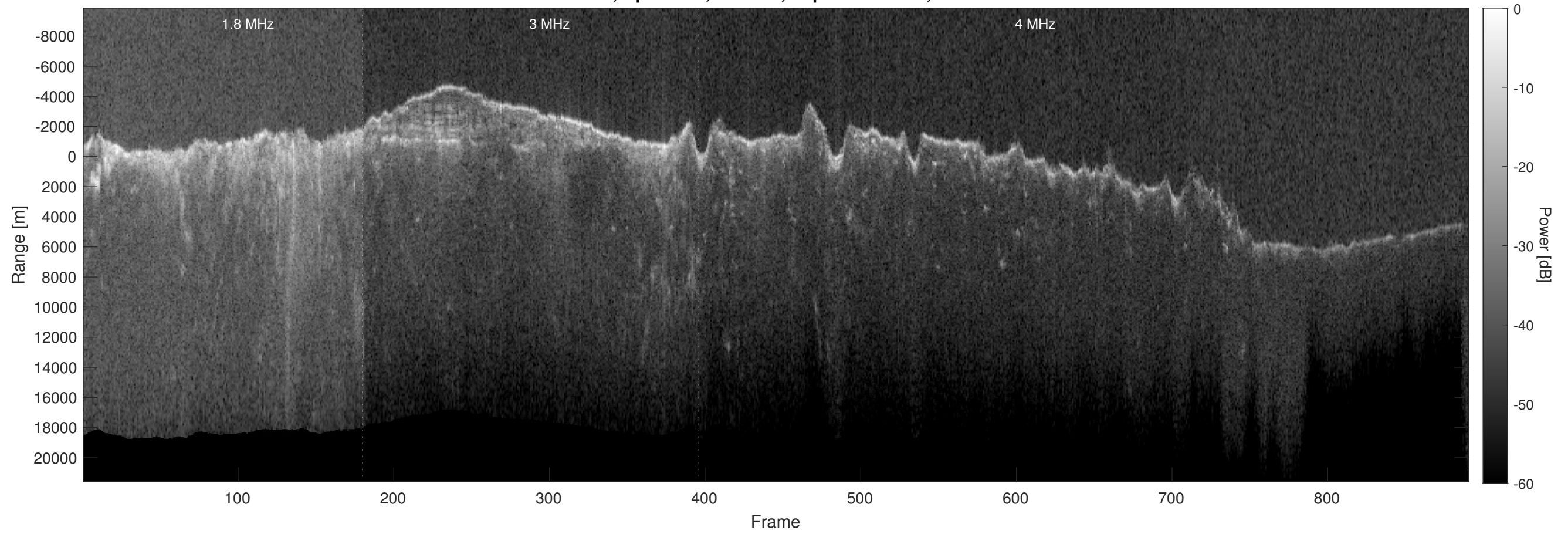
Orbit 8591, Optimized, Window, Depth-Corrected, Channel 2
