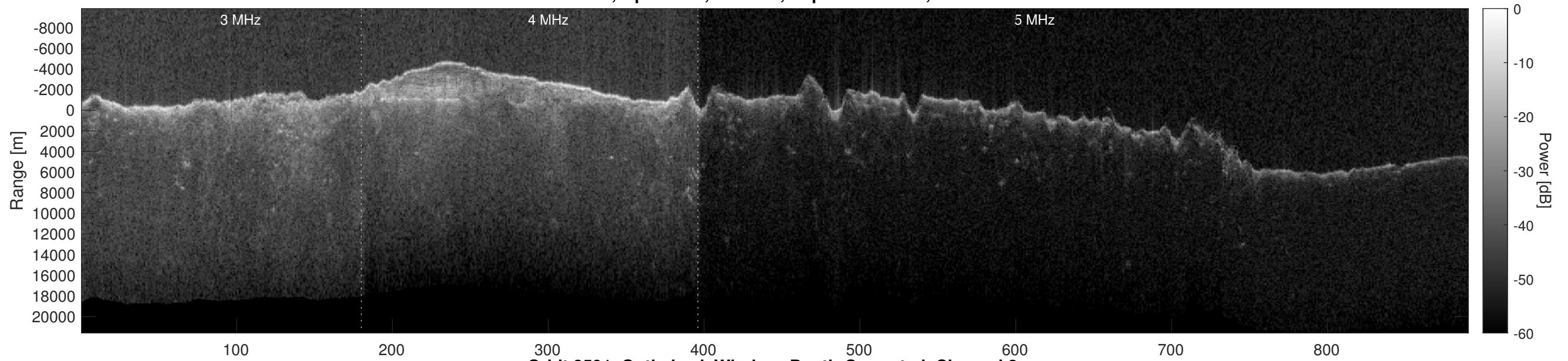
Orbit 8591, Optimized, Window, Depth-Corrected, Channel 2
