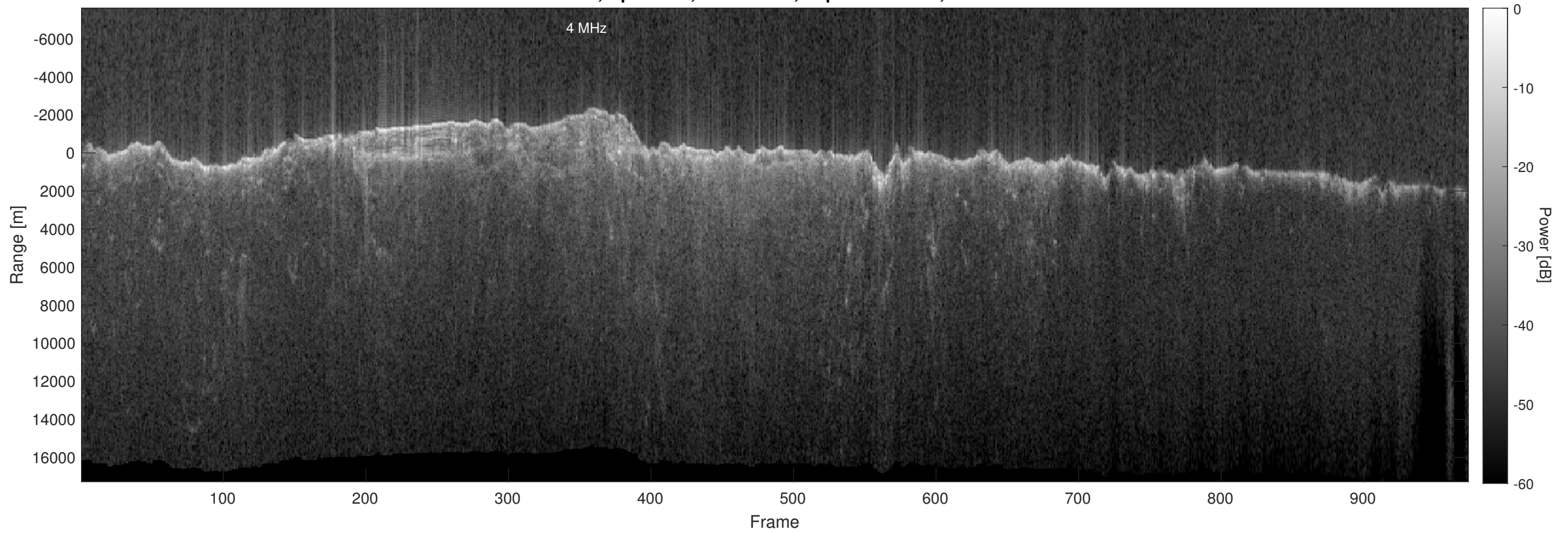
Orbit 8592, Optimized, No Window, Depth-Corrected, Channel 2
